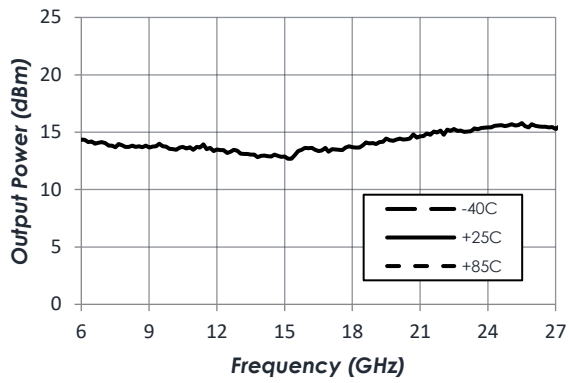
Power Saturation
